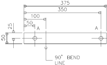
PART No 90g 6 No REQUIRED SCALE 1:5
