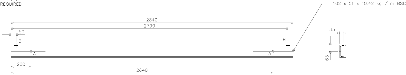
PART No 90b 2 No REQUIRED ELEVATION SIDE ELEVATION
