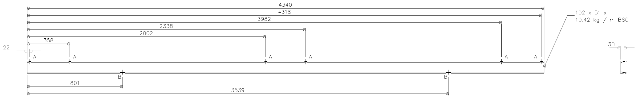
PART No 90b 2 No REQUIRED ELEVATION SIDE ELEVATION
