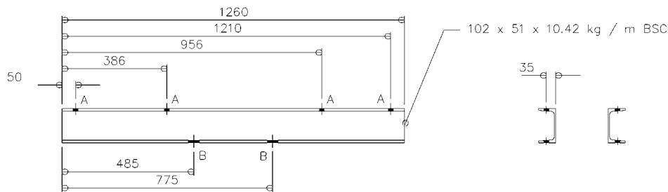
PART No 90d 1 PAIR REQUIRED ELEVATION SIDE ELEVATION
